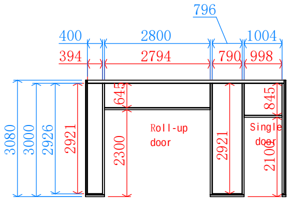
A View
